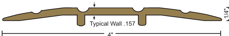
413BR 1.52 lbs./ft.
