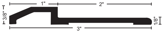
8138 .27 lbs./ft.
