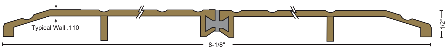
8428BR 3.62 lbs./ft.
